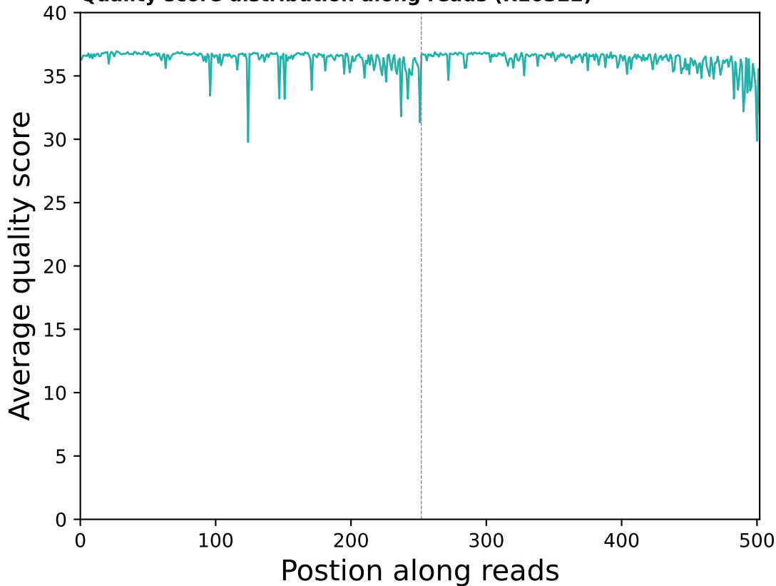
Quality score distribution along reads (R10322)
